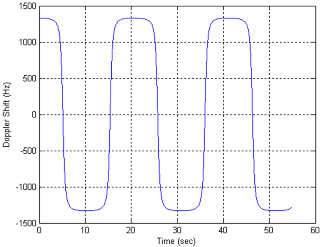
The Doppler shift trajectory for scenario 3 is shown in the following figure.
